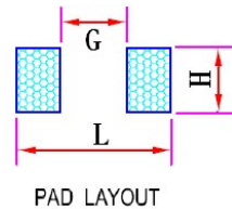
PAD LAYOUT
